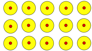
Figure 57: A simple model of a neutral material
