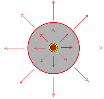
Figure 60: A polarised material
