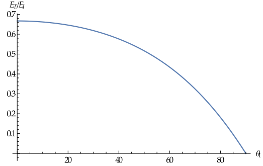
Figure 66: The transmitted field with normal polarisation
