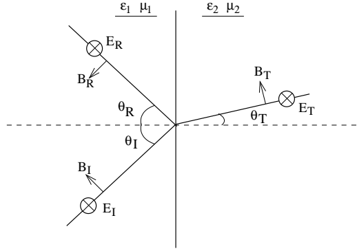
Figure 64: Incident, reflected and transmitted waves with normal polarisation.
