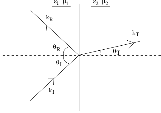
Figure 63: Incident, reflected and transmitted waves in a dielectric interface.
