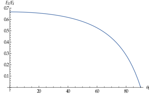
Figure 69: The transmitted field with parallel polarisation
