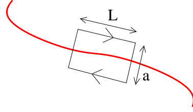
Figure 62: The tangential component of the electric field is continuous.
