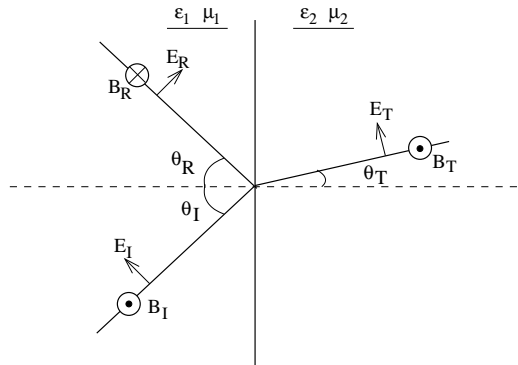
Figure 67: Incident, reflected and transmitted waves with parallel polarisation.
