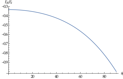
Figure 65: The reflected field with normal polarisation
