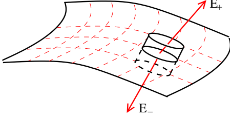
Figure 61: The normal component of the electric field is discontinuous
