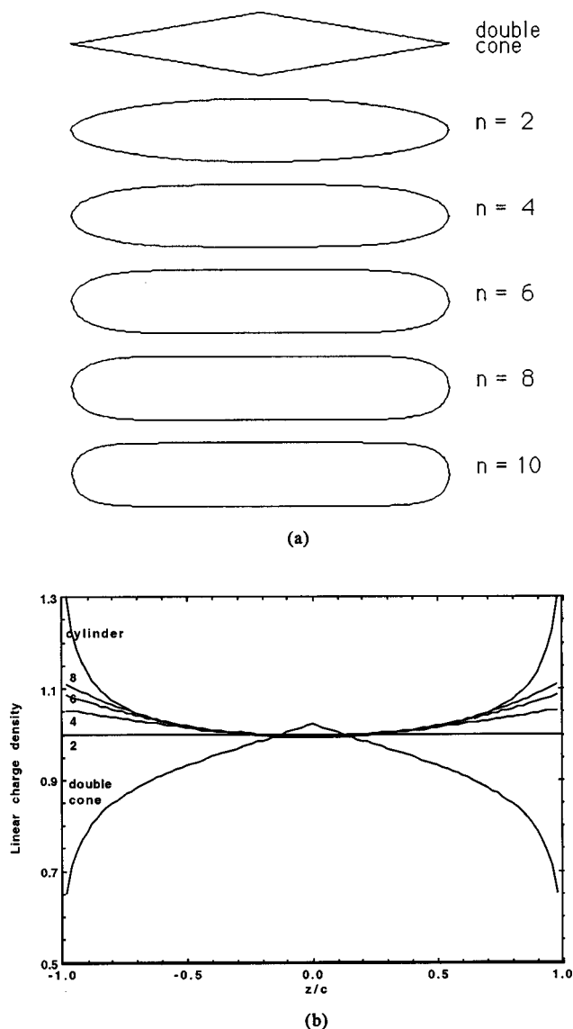
Fig. 4. (a) Shapes of conductors defined by r(z)/a = 1 - |z/c|^n [double cone] and r(z)^2/a^2 = 1 - |z/c|^n . The transverse (radial) coordinate has been scaled by a factor of c/6a to make the different shapes visible. (b) Linear charge densities for the shapes of part (a) for the double cone and n=2,4,6,8 for \Lambda=15 , along with that of a right circular cylinder. Note the suppressed zero for the ordinate.
