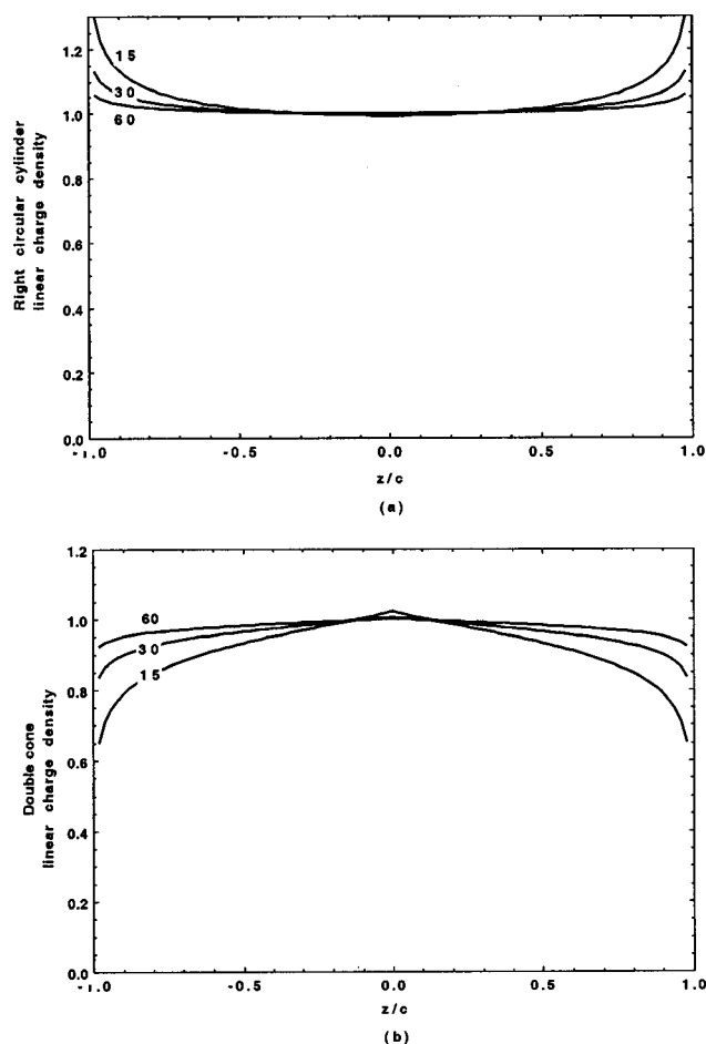
Fig. 5. Behavior of the linear charge density versus z/c with increasing \Lambda ( \Lambda=15,30,60 ) for two different shapes. (a) Right circular cylinder. (b) Double cone.
